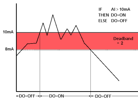
Figure 4-10 : AI Deadband Operation(> or \geq a numerical value)
